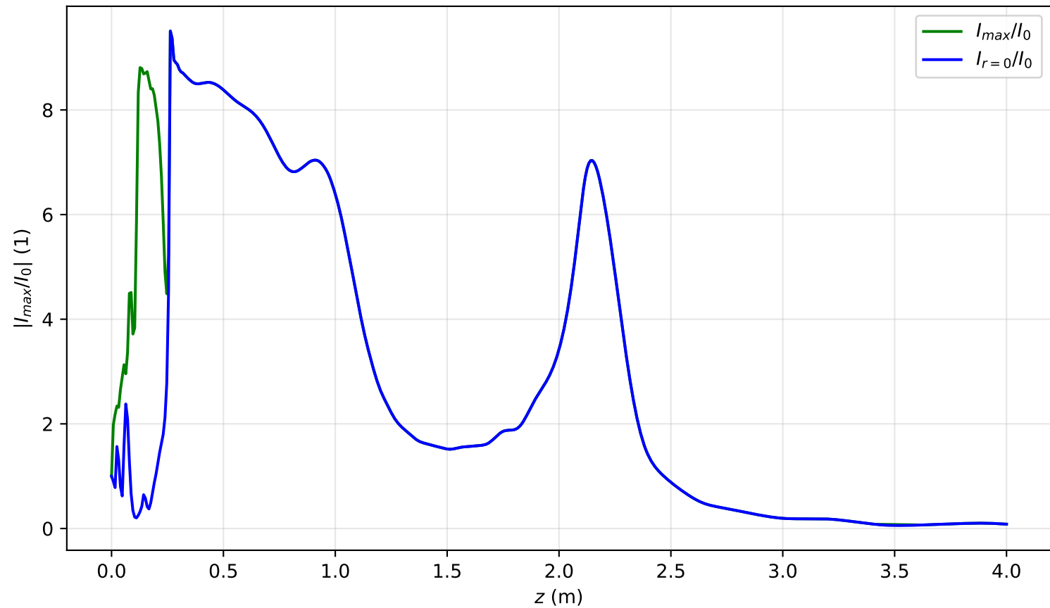
I_{\max}(x = 0, y = 0, z)/I_0 , Pin=8.0Pcr, artificial time
